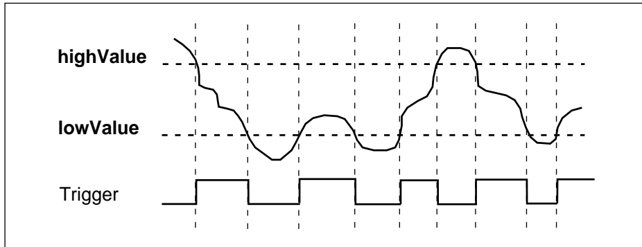
Figure 2-6. ND_INSIDE_REGION
