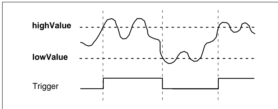
Figure 2-7. ND_HIGH_HYSTERESIS
